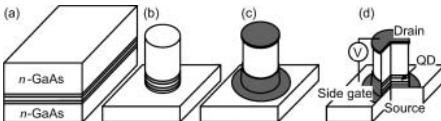
Figure 4.6 Fabrication process of a VQD consists mainly of (a) epitaxial growth of a BDH, (b) etching of a pillar through the DBH, and (c) the metallization (following Ref. 19). The QD of the device is defined by the DBH and the side gate. (d) The final device.
