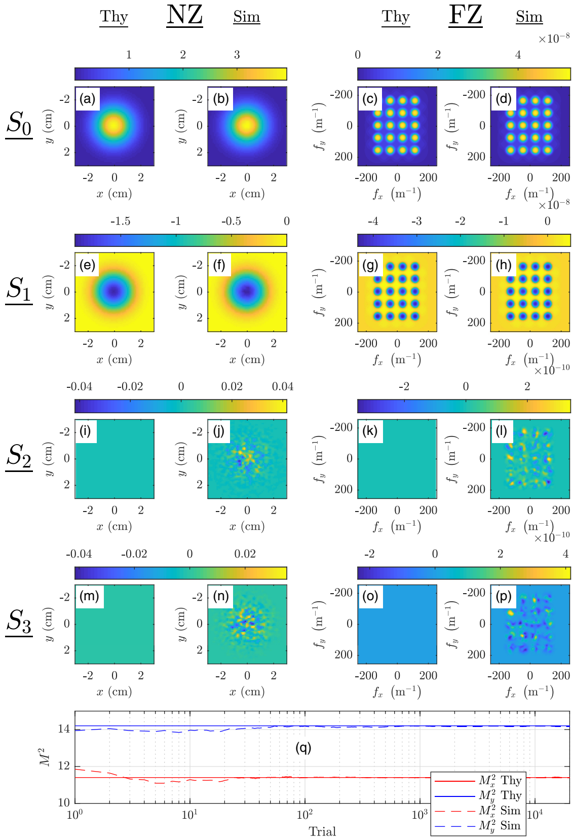
Fig. 2 VOCL results—(a) S_0^{\text{NZ}} Thy, (b) S_0^{\text{NZ}} Sim, (c) S_0^{\text{FZ}} Thy, (d) S_0^{\text{FZ}} Sim, (e) S_1^{\text{NZ}} Thy, (f) S_1^{\text{NZ}} Sim, (g) S_1^{\text{FZ}} Thy, (h) S_1^{\text{FZ}} Sim, (i) S_2^{\text{NZ}} Thy, (j) S_2^{\text{NZ}} Sim, (k) S_2^{\text{FZ}} Thy, (l) S_2^{\text{FZ}} Sim, (m) S_3^{\text{NZ}} Thy, (n) S_3^{\text{NZ}} Sim, (o) S_3^{\text{FZ}} Thy, (p) S_3^{\text{FZ}} Sim, and (q) convergence of simulated M_x^2 and M_y^2 to the corresponding theoretical values versus trial number.
