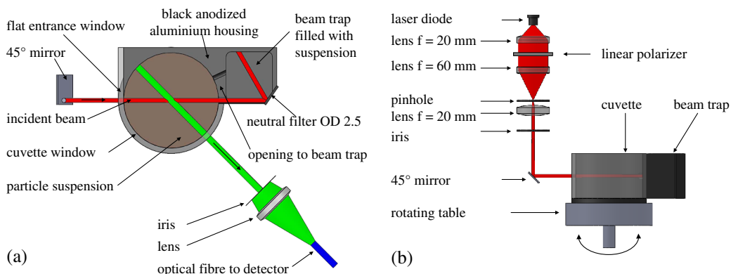
Fig. 5 (a) The cuvette and (b) the illumination setup for creating a collimated beam ( \varnothing 2 = \text{mm} ) for illumination of the cuvette. The illumination setup is fixed to the cuvette.
