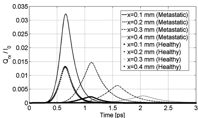
Fig. 6 Evolution of dimensionless radiative flux (diffuse component) in the middle position of the medium along the (Ox) axis.
