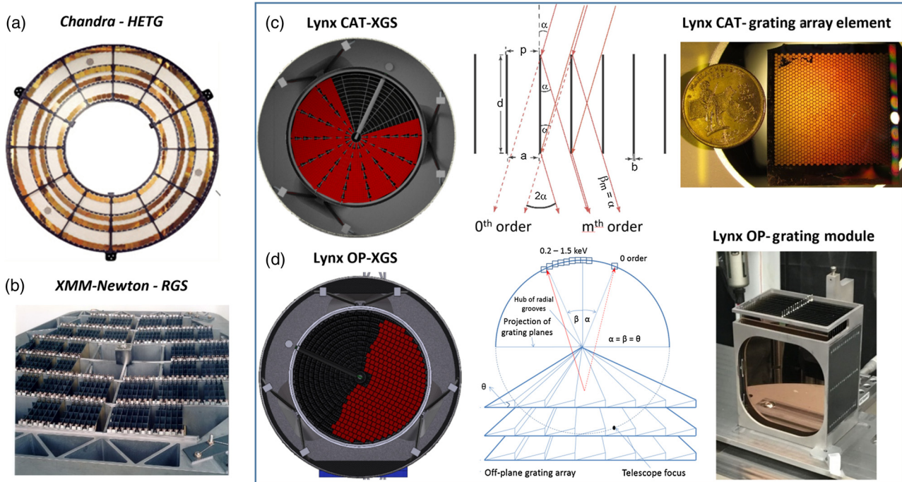
Fig. 12 (a) Images of Chandra’s HETG and (b) XMM-Newton’s RGS. These large-scale structures have been successfully operating for over 20 years on orbit. Like these instruments, Lynx will use either transmission (c) or reflection (d) gratings, but using different technologies, and will require a much larger grating effective area. Depending on the technology selected for Lynx, different mirror coverages may be required. The current design requires ~73% mirror coverage of the CAT gratings (baseline for the DRM), and ~50% coverage for the OP gratings (credit: Chandra HETG/NASA, XMM-Newton RGS/ESA, Lynx CAT- and OP-XGS drawings/NASA, Lynx CAT-XGS image/MIT, and OP-XGS image/PSU).
