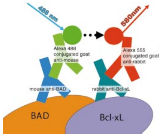
Fig. 1 BAD and Bcl-xL heterodimerization. The heterodimerization of BAD labeled with Alexa 488 and Bcl-xL labeled with Alexa 555 approximates the fluorophores within 100 Å of each other, enabling fluorescent resonance energy transfer.
