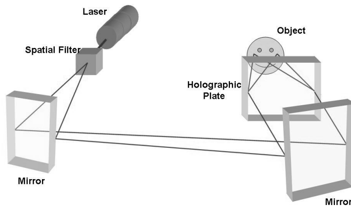
Fig. 11. Holographic experimental set-up. Denisyuk's configuration.
