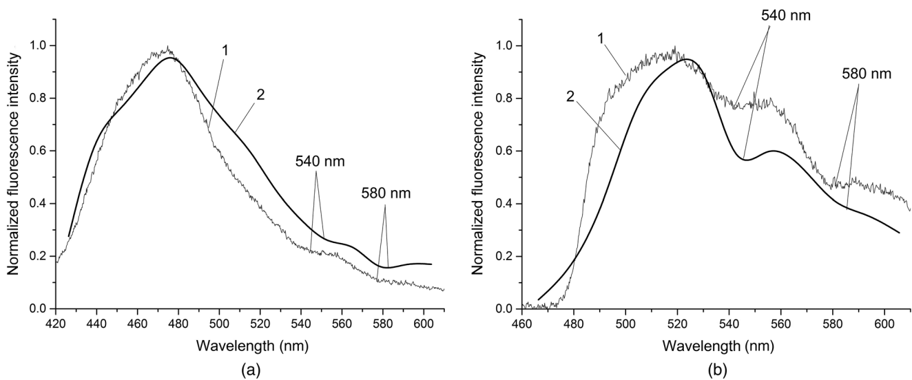
Fig. 5 Comparison of (1) experimental and (2) model-based spectra, calculated using the Monte-Carlo method. Model simulates presence of (a) NADH + collagen and (b) FAD + collagen.
