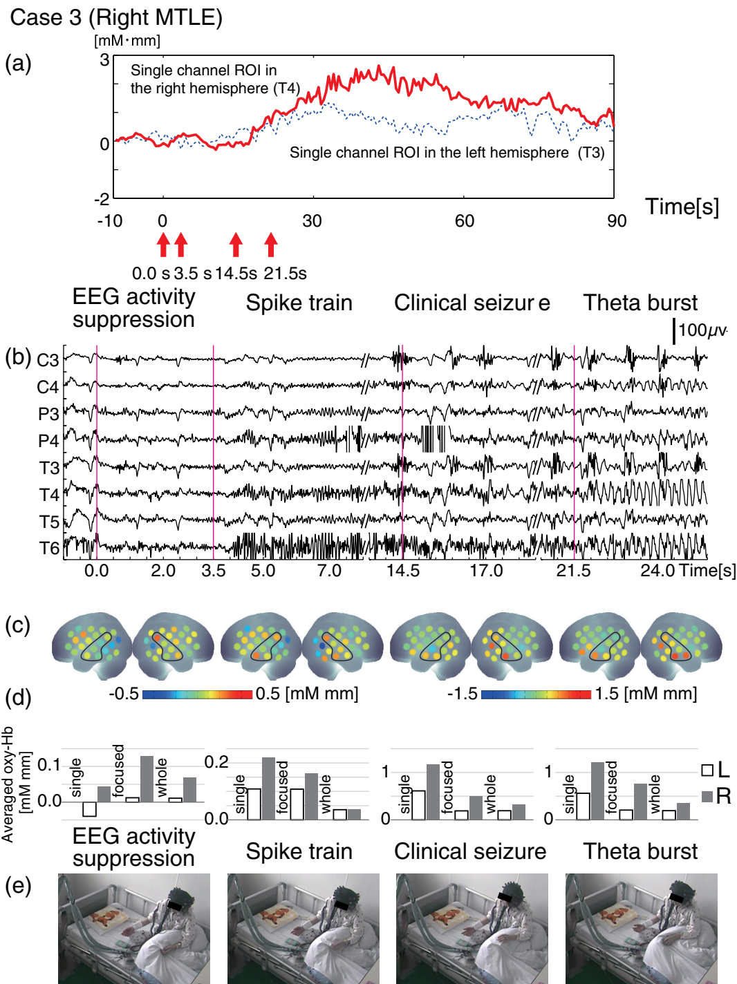
Fig. 5 EEG and fNIRS data during the seizure of case 3. Figure details as for Fig. 3.
