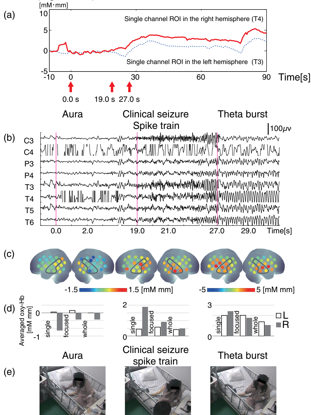
Fig. 6 EEG and fNIRS data during the seizure of case 4. Figure details as for Fig. 3.
