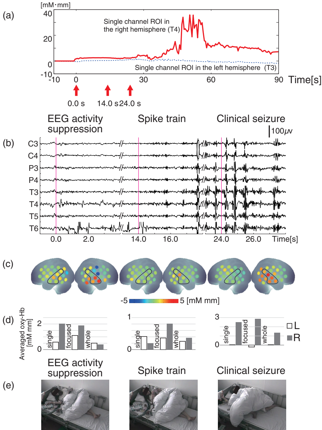
Fig. 3 EEG and fNIRS data during the seizure of case 1. (a) Oxy-Hb signals at the two single-channel ROIs around the EEG channels of T3 and T4. Epileptic focus side is indicated with the solid red line and the contralateral side is indicated with the dotted blue line. The characteristic events are indicated with red arrows. (b) EEG data for channels covering the focused area as determined by fNIRS channels. The characteristic events are indicated with vertical red lines. (c) Colored brain maps of fNIRS activations at the times of characteristic events. The focused area is enclosed with a black line. (d) The period-average values of oxy-Hb 20s after the characteristic events. The channel groups, from left to right, are the single-channel area, the focused area, and the whole-hemisphere area. Focus side values are indicated with gray bars and contralateral side values are indicated with white bars. (e) Still captures taken from the video, which was simultaneously recorded.
