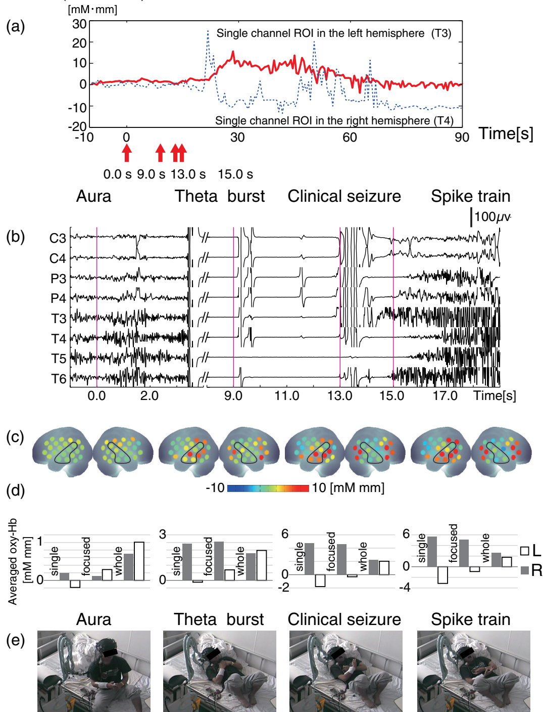
Fig. 4 EEG and fNIRS data during the seizure of case 2. Figure details as for Fig. 3.
